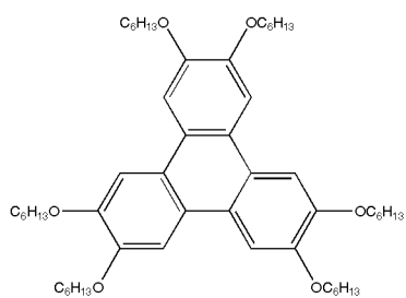
Triphenylene (HAT6)
