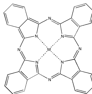
Phthalocyanine
