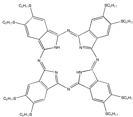
Phthalocyanine
